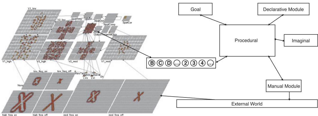
Fig. 3. The combined Leabra and ACT-R architecture as used for the Attentional Blink model, in which the Leabra neural network replaces ACT-R's visual module.
