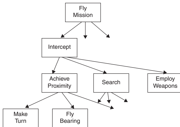
Fig. 1. Example of part of the goal hierarchy of TacAir-Soar.
